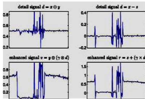
Fig.4.2:Illustration of the difference between the proposed generalized unsharp masking algorithm (left panel) and the classical unsharp masking algorithm (right panel).
