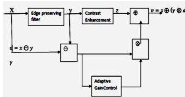
Fig.4.1: Block diagram of the proposed generalized unsharp masking algorithm
