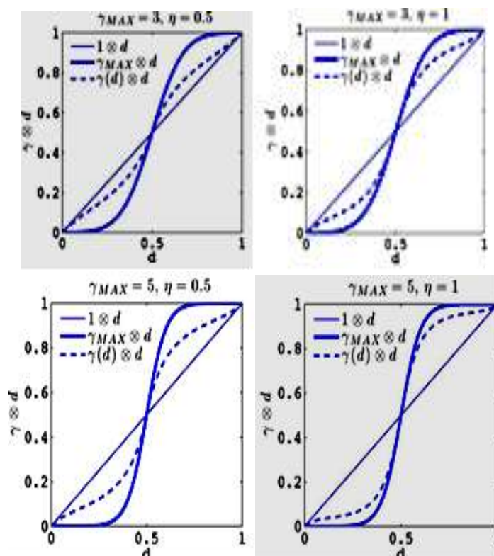
Fig.4.3: Illustrations of adaptive gain control for four combinations of \eta and \gamma_{max}
