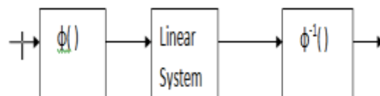
Fig 3.1: Block diagram of a generalized linear system, where \phi() is usually a nonlinear function.
